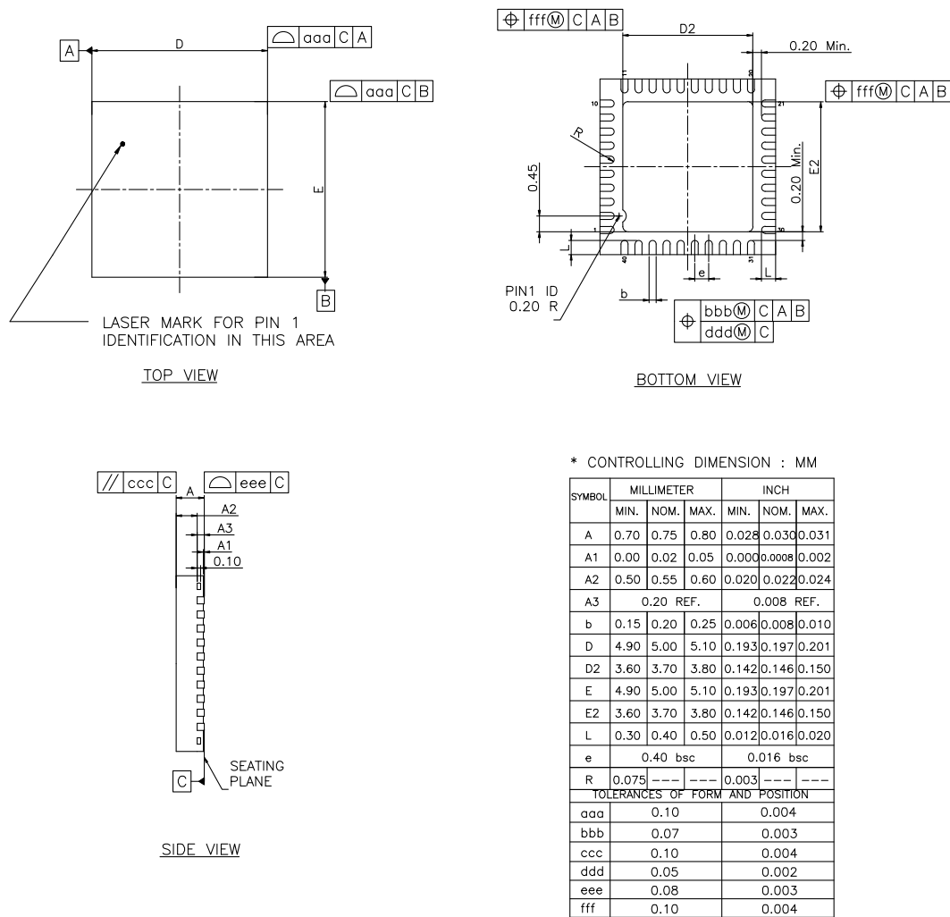
Figure 8-1 QFN40 Mechanical Parameters
