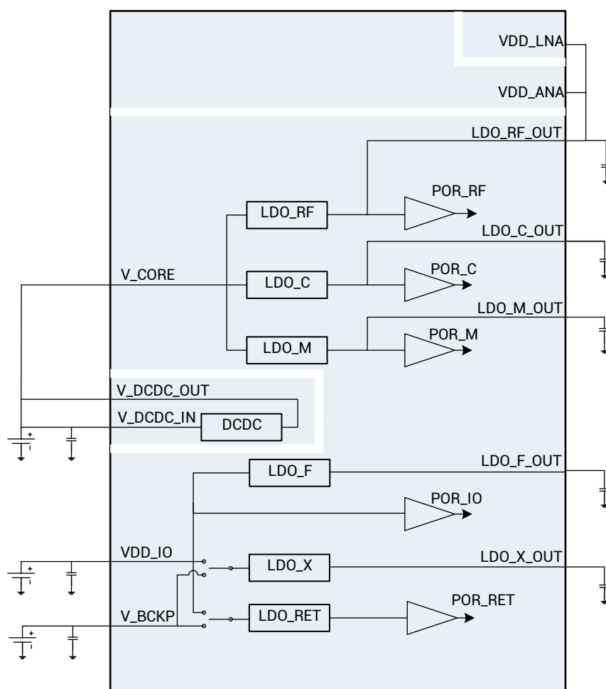
Figure 5-1 Power-on and sequence of DC/DC bypass (Main Supply is 1.2V ~ 1.98V)
